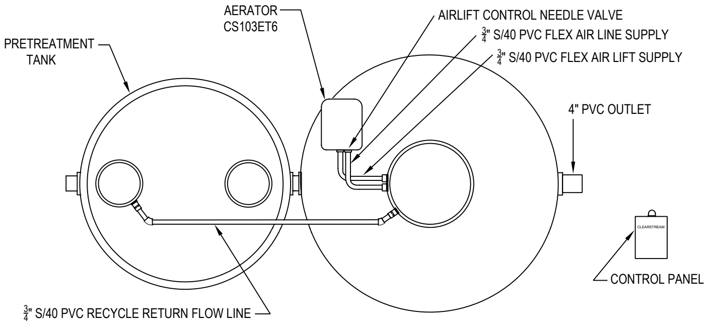
PLAN
