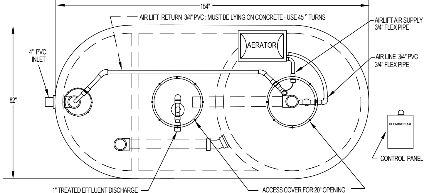
PLAN
