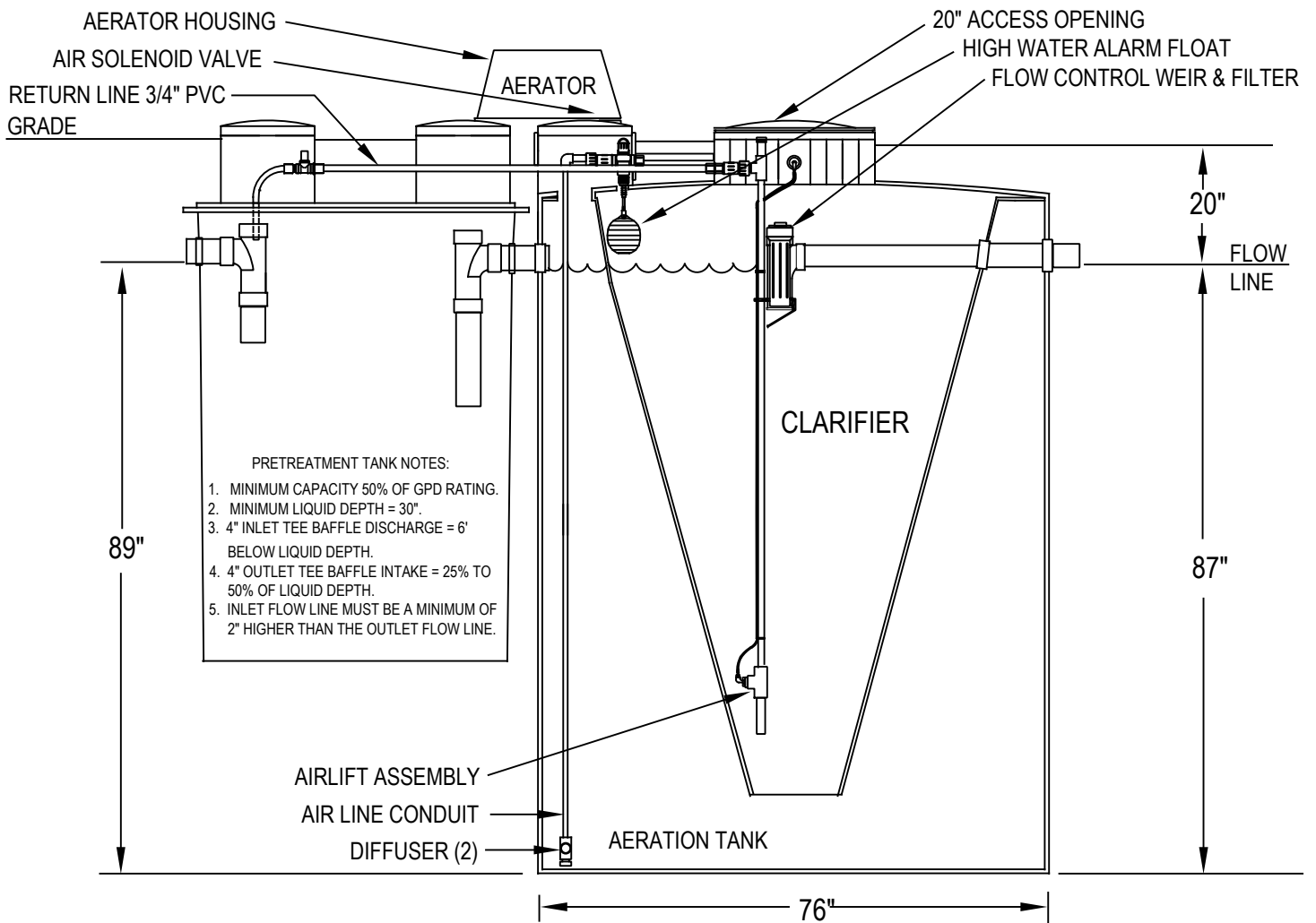
SECTION
